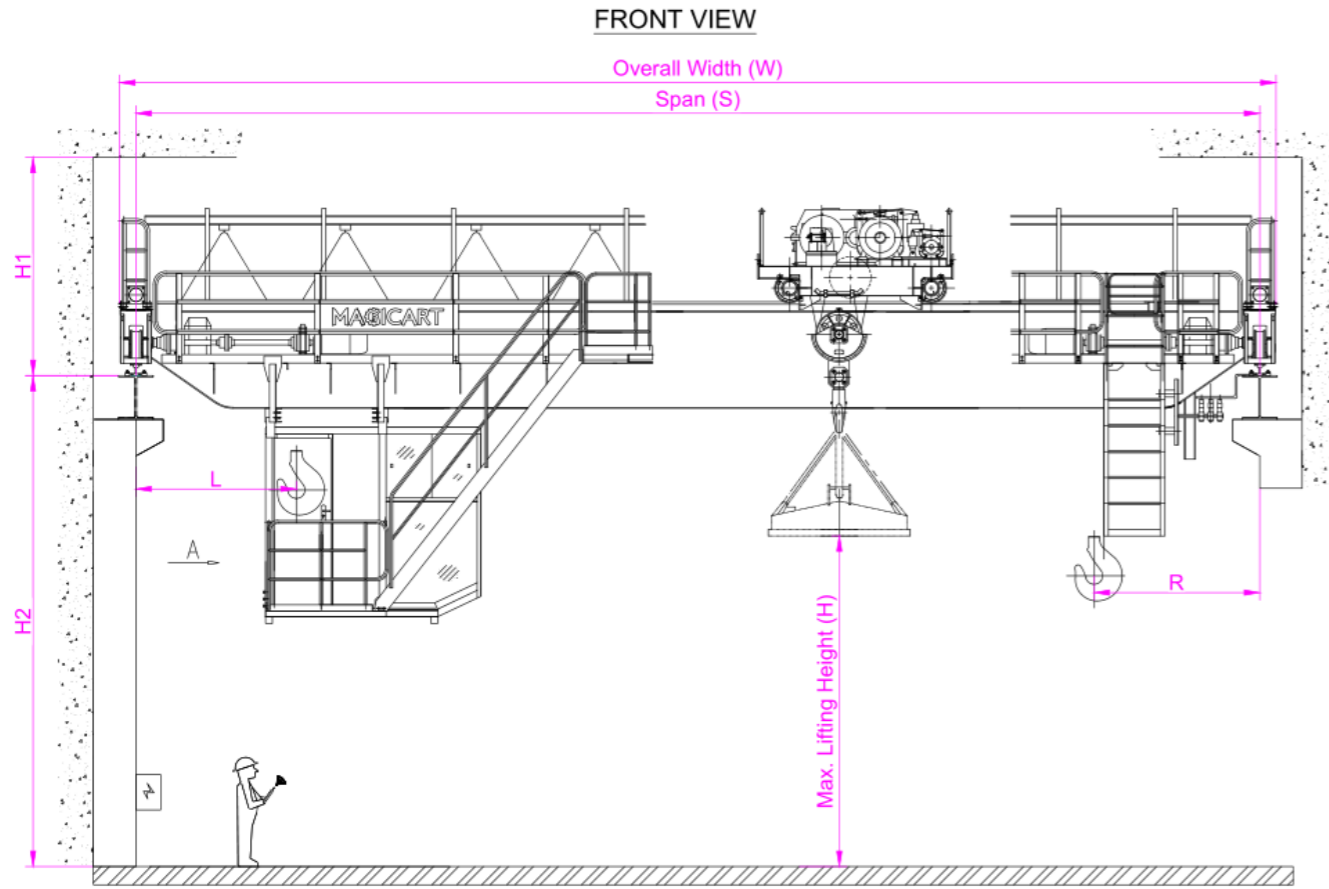
CRANE LAYOUT
