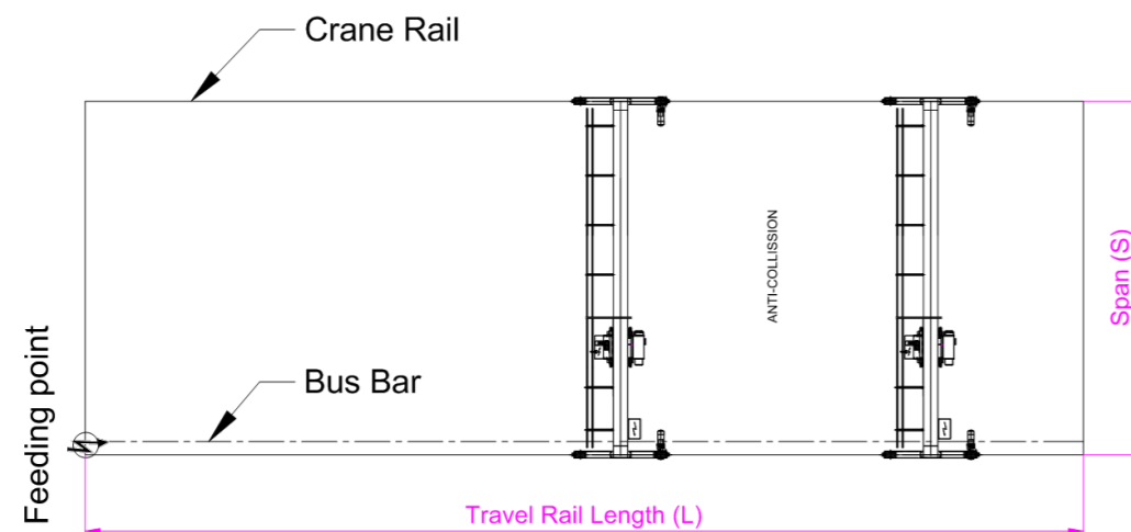
CRANE LAYOUT
