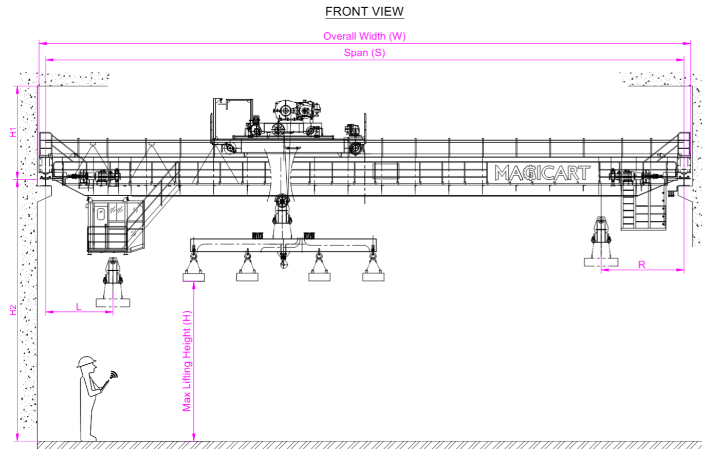
CRANE LAYOUT
