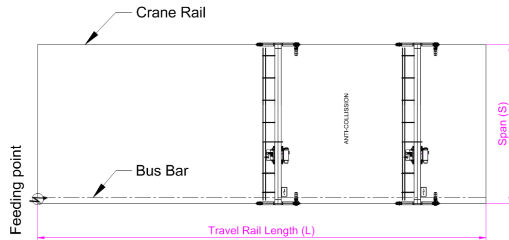
CRANE LAYOUT
