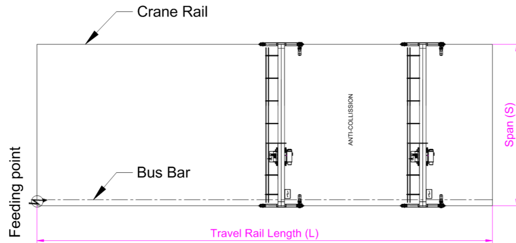
CRANE LAYOUT
