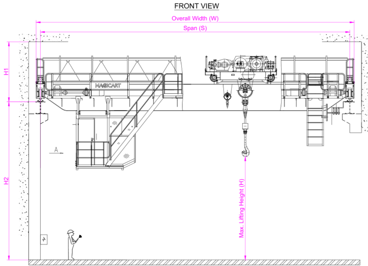
CRANE LAYOUT
